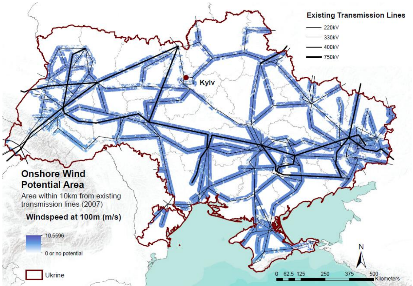
Figure 5: Scenario 2 – onshore wind potential in the Ukraine - Restriction based on proximity to electricity transmission lines
