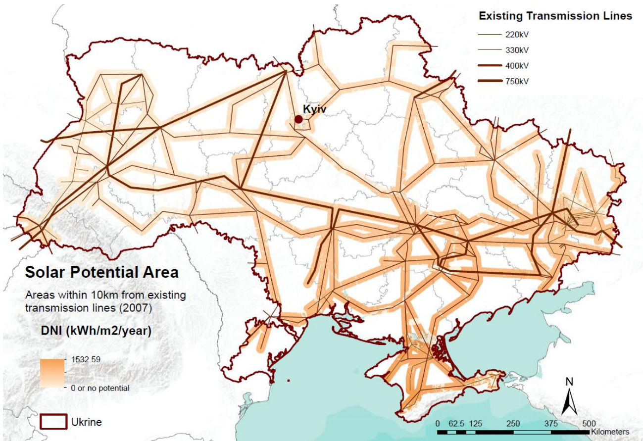
Figure 3: Scenario 2 - solar potential in the Ukraine - Restriction based on proximity to electricity transmission lines
